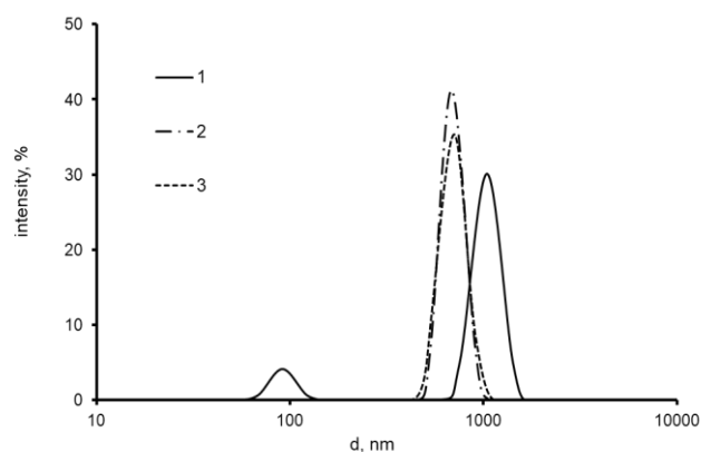
Figure 4. Size distribution ( d ) by intensity curves of lecithin aggregates in distilled water (1) and in the presence of the natural water from Don (2) and Usman (3) rivers (Voronezh nature reserve).
