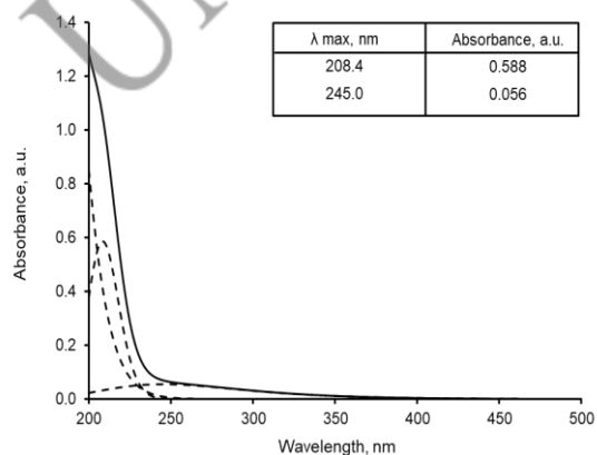
Figure 1. UV-spectrum of water from the Don river and its Gaussian. (here and further: solid curve is initial and calculate spectra, dotted lines are its Gaussian)
