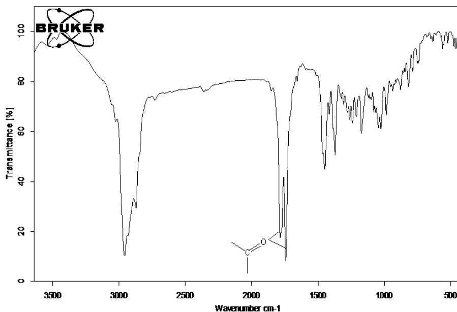
Figure 1S. FTIR spectrum of essential oils from Artemisia herba-alba L.
