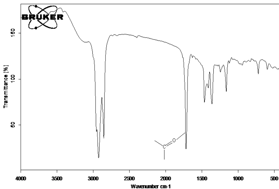
Figure 2S. FTIR spectrum of essential oils from Ruta montana L.
