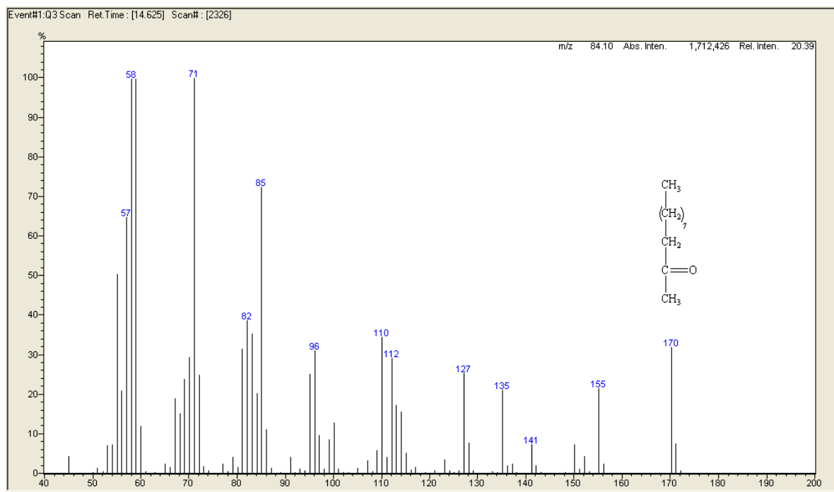
Figure 7S. Mass spectrum of 2-undecanone.
