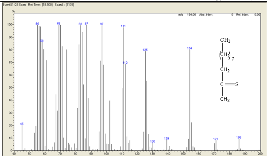
Figure 8S. Mass spectrum of 2-undecanethione.
