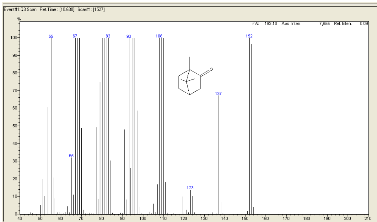
Figure 5S. Mass spectrum of camphor.
