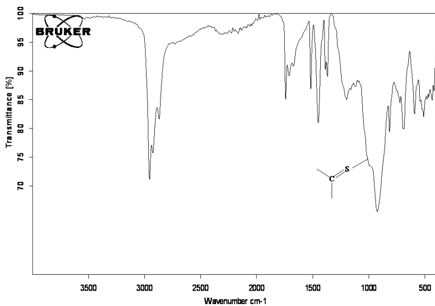
Figure 3S. FTIR spectrum of thionated essential oils from Artemisia herba-alba L.
