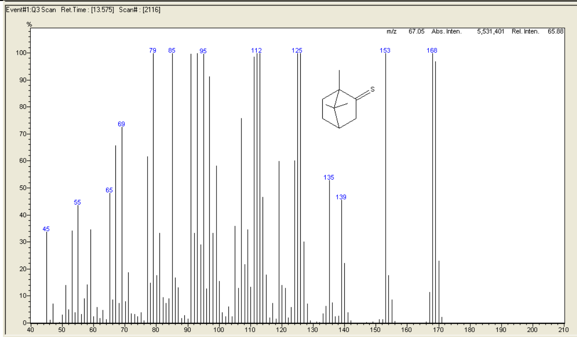
Figure 6S. Mass spectrum of thioamphor.
