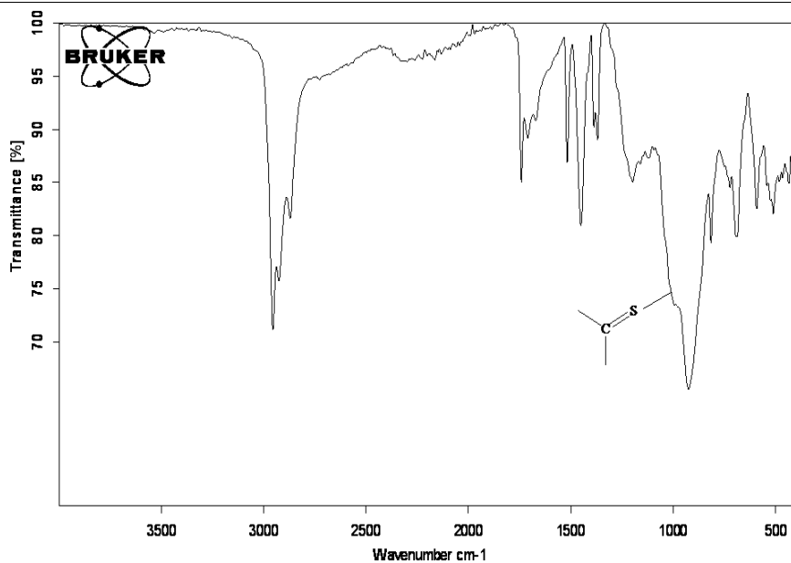
Figure 4S. FTIR spectrum of thionated essential oils from Ruta montana L.
